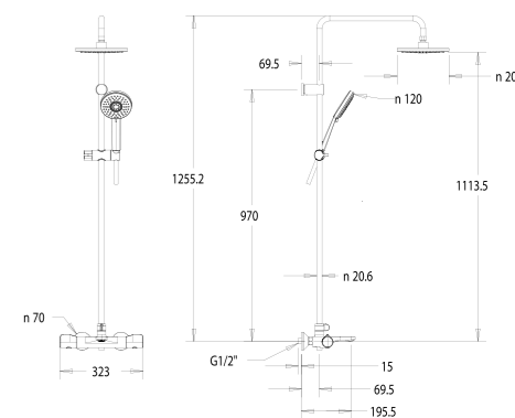
TEMPTACION™ Exposed Auto Temperature Shower System (3-way)
